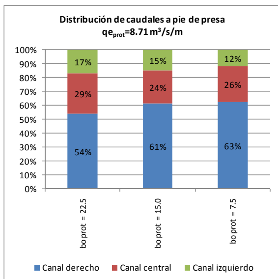
Ilustración 4. q_{e \text{ prot}} = 8.71 \text{ m}^3/\text{s}/\text{m}
