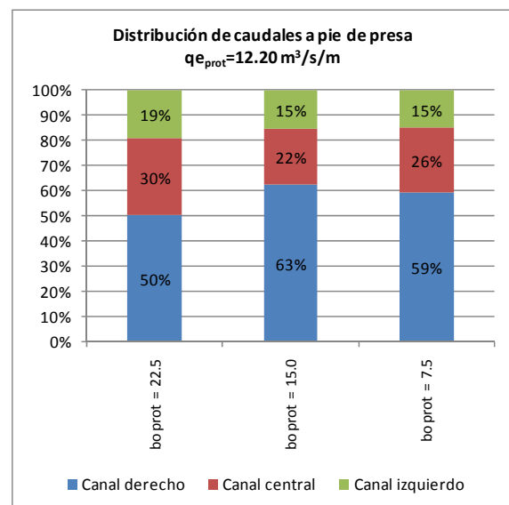
Ilustración 5. q_{e \text{ prot}} = 12.20 \text{ m}^3/\text{s}/\text{m}
